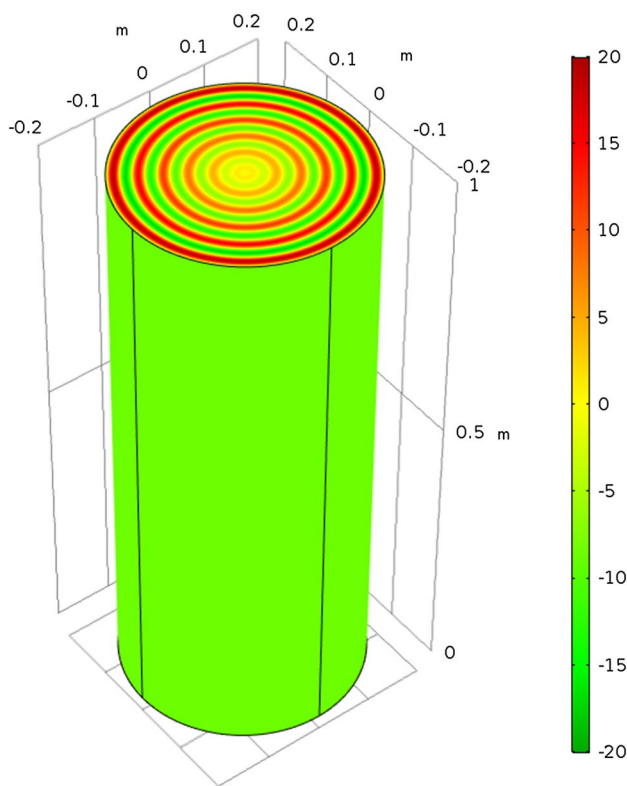
Fig. 6 Example of a finite element model trunk in the case of an interlocked grain pattern. Colour levels indicate grain angles ranging from -20^\circ (green) to +20^\circ (red)
