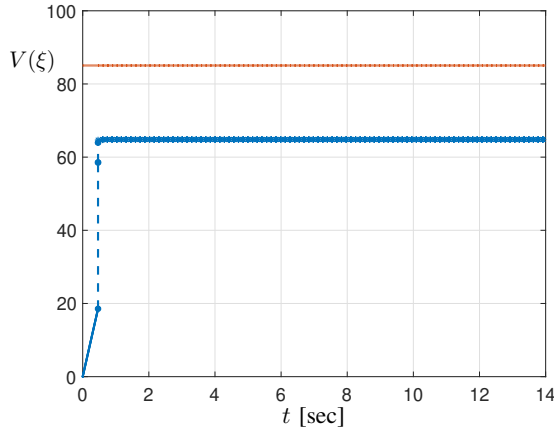
Fig. 2: The evolution of the function \tilde{J}_\phi in Example 1.
