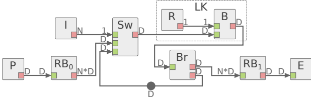
Figure 7: Equivalent SDF graph of Algorithm 1.
