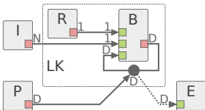
Figure 8: Equivalent SAD graph of Algorithm 1.
