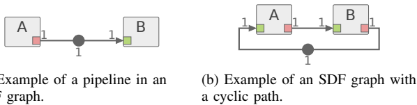
Figure 3: Examples of delay usage in dataflow graphs.
