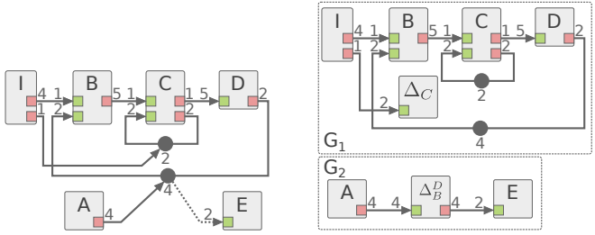
(a) An SDF graph with the proposed semantics of delays.
