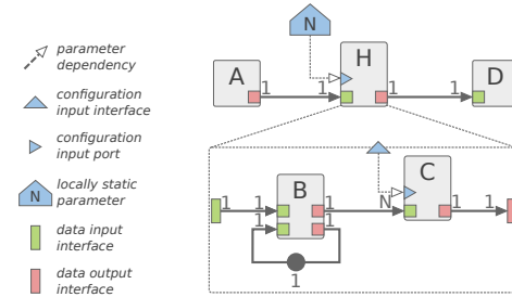
Figure 2: Example of a \pi SDF graph.
