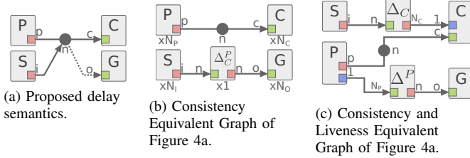
Figure 4: Proposed semantics of delay and equivalent graphs used for consistency and liveness analyses.
