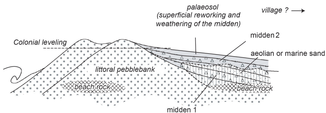
Figure 2. Interpretative section of the Gare Maritime site representative of the Pre-columbian period (modified after Bertran P. in Romon, 2013).
