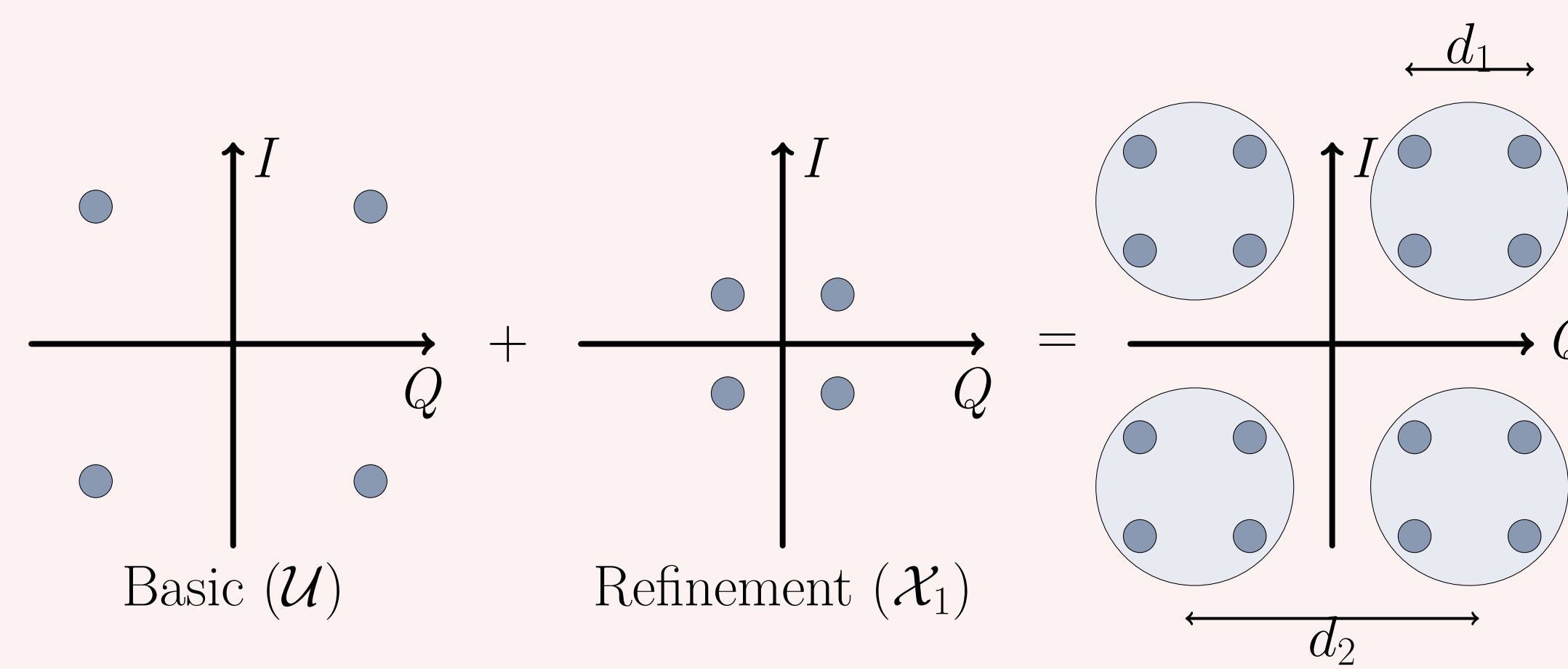
Figure 3: Hierarchical Modulation
