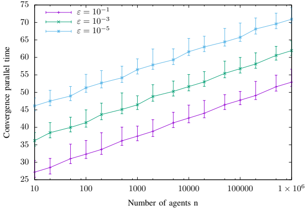
Figure 8. Parallel convergence time of Proportion Computation with Convergence Detection as a function of n , with N = 10^3 .
