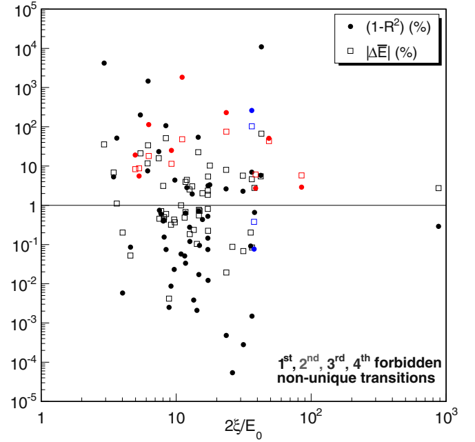
FIG. 1. (Color online) Distribution according to 2\xi/E_0 of the (1 - R^2) and |\Delta\tilde{E}| parameters for the measured shape factors of forbidden nonunique transitions.
