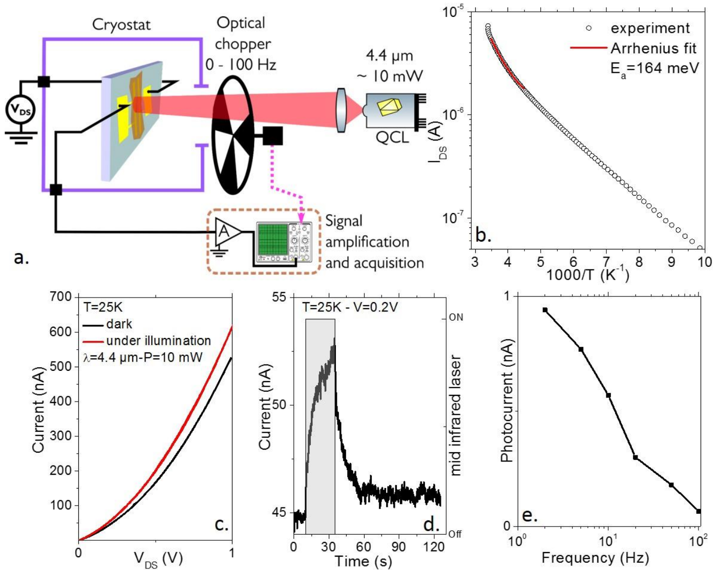
Figure 5 a. Scheme of the setup used for the illumination of the sample by a mid-IR source (ie a quantum cascade laser operated at 4.4 \mu\text{m} with a 10 \text{ mW} power, Reprinted with permission from ref 38 (2018) American Chemical Society. b. Dark current under 1\text{V} as a function of the temperature for a film made of small \text{Ag}_2\text{Se} CQDs. c. IV curve for a film made of small \text{Ag}_2\text{Se} CQDs under dark condition and under illumination by the quantum cascade laser. d. Current as function of time while the mid-IR source is turned on and off. e. Bode diagram (photocurrent as a function of signal frequency) for a film made of small \text{Ag}_2\text{Se} CQDs.
