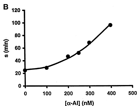
Fig. 3. Lineweaver–Burk plot using maltopentaose as substrate. (A) Reciprocal plots obtained with variable maltopentaose concentrations and at fixed concentration of the Phaseolus inhibitor α-AI. The reciprocal plots are drawn from one set of data. (B, C) Secondary plots showing the dependence of the vertical axis intercept ( i ) and of the slope ( s ) on the concentration of Phaseolus inhibitor α-AI.
