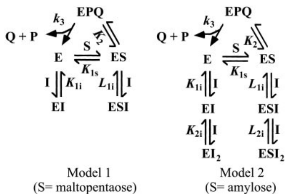
Fig. 4. Two models proposed for the noncompetitive inhibition of PPA-catalysed amylose (model 1) and maltopentaose (model 2) hydrolysis. P and Q are products. K and L are dissociation equilibrium constants and k_3 a rate constant.
