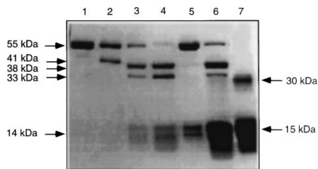
Fig. 1. SDS/PAGE analysis. PPA (lane 1), PPA-subtilisin 2% (lane 2), \alpha -AI (lane 7), PPA- \alpha -AI at an \alpha -AI/PPA ratio of 1 (lane 5), PPA- \alpha -AI-subtilisin 2% with an \alpha -AI/PPA ratio of 0.4 (lane 3), 1 (lane 4) and 10 (lane 6). Loading: 1.5 \mu g protein per well. The molecular masses indicated on each side come from protein marker migration (not shown).
