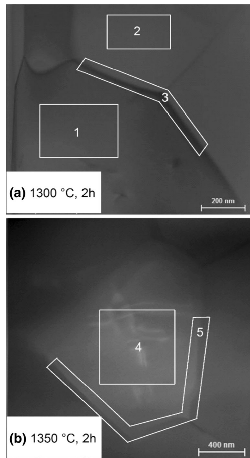
Fig. 4 Bright field TEM images of ceramics sintered at several temperatures. Areas analysed by EDS are shown
