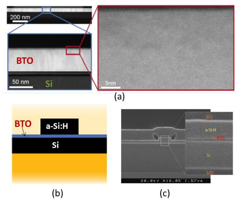
Figure 1: (a) Results on the integration of 50 nm BaTiO 3 on Si by molecular beam epitaxy (MBE); (b) Schematic and (c) SEM image of the slot BaTiO 3 /Si waveguide.
