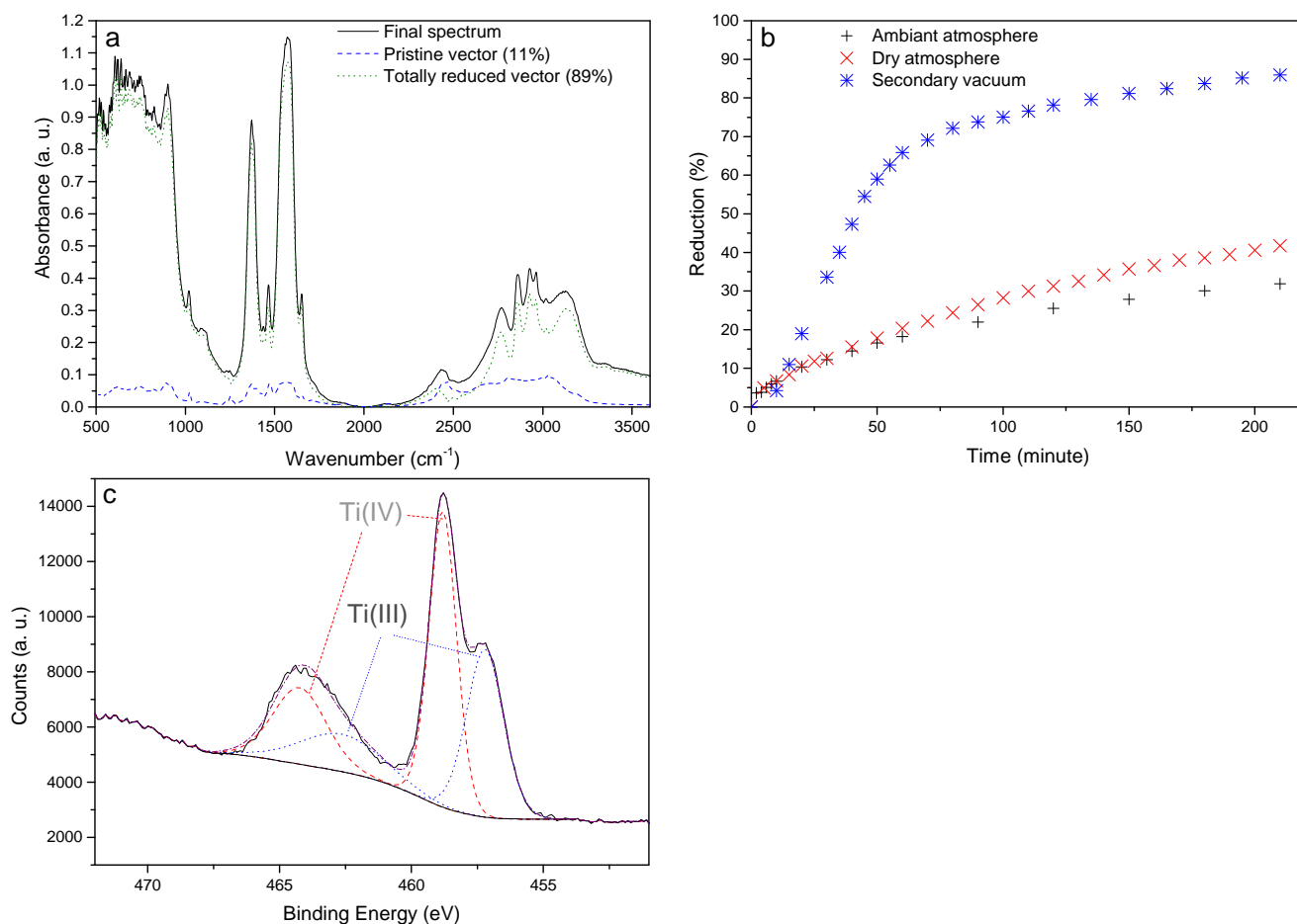
Fig. 3. Infrared spectrum after 4 h of illumination (line) with its decomposition (pristine vector in dash and totally reduced vector in dot) under secondary vacuum atmosphere (a.); Evolution of the reduced vector percentage in the Infrared spectra fits under different atmospheres (b.); XPS spectrum of Ti 2p for an TiDMF layer reduced for 5 h30 with the contribution of Ti(IV) and Ti(III) under ambient atmosphere (c.) (For interpretation of the references to colour in this figure legend, the reader is referred to the web version of this article.)
