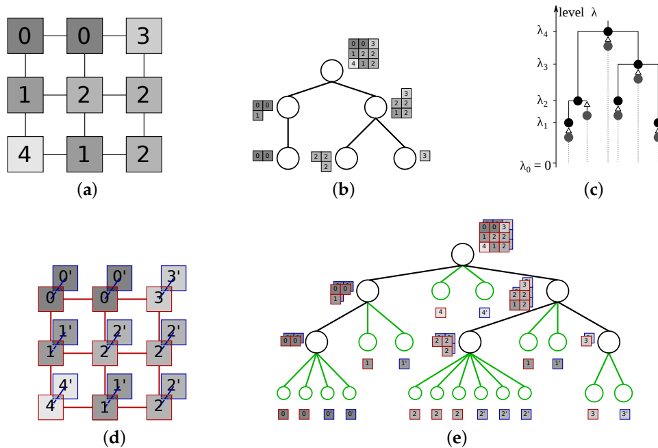
Figure 4. A possible inclusion tree for the image displayed in (a) is shown in (b), with one possible dendrogram shown in (c). In this dendrogram, the gray nodes with \triangle represent new image elements entering the hierarchy, and do not belong to the support before then as indicated by the gray dotted line. The image extended by ghost pixels is shown in (d), with the links between original pixels shown in red and the links between the ghost and corresponding original pixels in violet. The extended tree shown in (e) is a partitioning tree for (d), with the auxiliary nodes (in green) identifiable as the singletons in the hierarchy.
