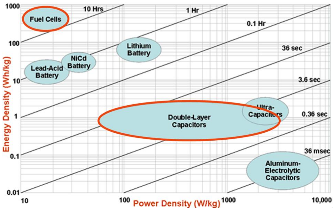
Figure 1 : Ragone plot of various energy devices and their charge times (diagonal strokes) [7].
