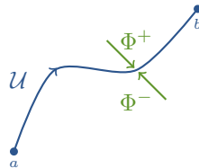
Figure 12: Left and right limits on the open contour \mathcal{U}
