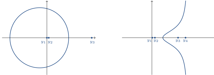
Figure 9: The curve \mathcal{L} for Gessel's model (on the left) and for the model with jumps \{E, N, SW, S\} (on the right), for t = 1/8
