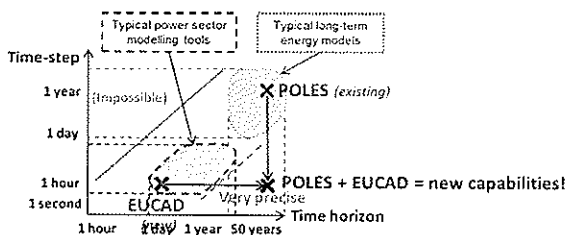
Fig. 1. Typical time scales and time steps simulated in the coupling of EUCAD and POLES
