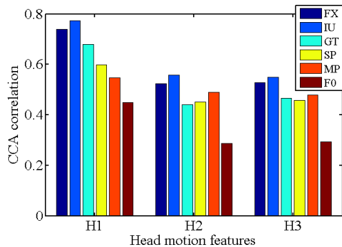
Fig. 2. Correlation of CCAs between each of H1, H2, H3 and FX, IU, GT, SP, MP and F0
