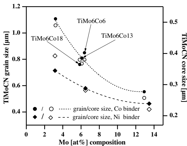
Fig. 5. Average grain size (core + rim) and core size of TiMoCN grains as a function of the Mo content in raw powders.
