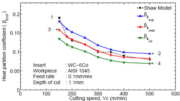
Figure 4: Evolution of heat partition coefficient vs cutting speed for different conductivity values
