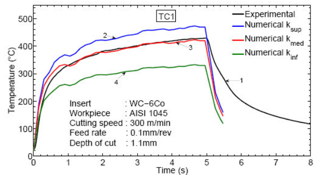
Figure 9: Comparison of experimental (1) and numerical temperatures (2, 3, 4) for different conductivity values (Thermocouple TC1).
