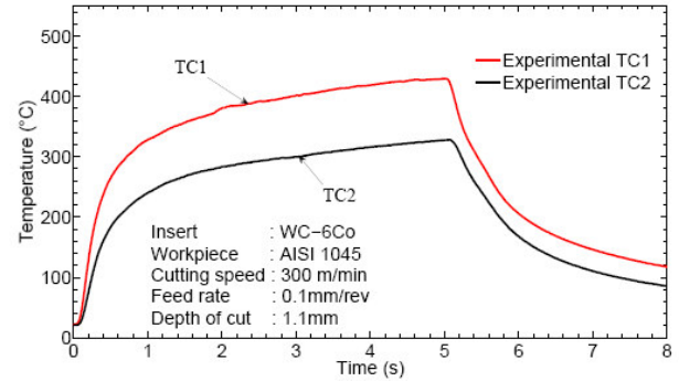
Figure 6: Evolutions of the cutting tool temperature vs time ( V_c = 300 m/min)
