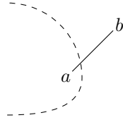
Fig. 8: Case 2: The vertex a is part of only one 2-edge \{a, b\} and may be part of other 3-edges.
