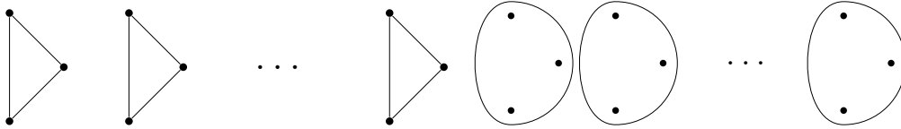
Fig. 1: Moon and Moser's construction (left) and its analogue for (3, 3) -hypergraphs (right).
