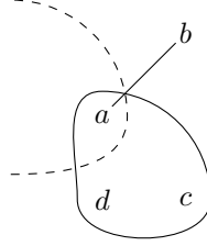
Fig. 9: Case 2.2: The vertex a is part of only one 2-edge \{a, b\} and at least one 3-edge \{a, c, d\} .
