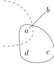
Figure 9: Case 2.2: The vertex a is part of only one 2-edge \{a, b\} and at least one 3-edge \{a, c, d\} .
