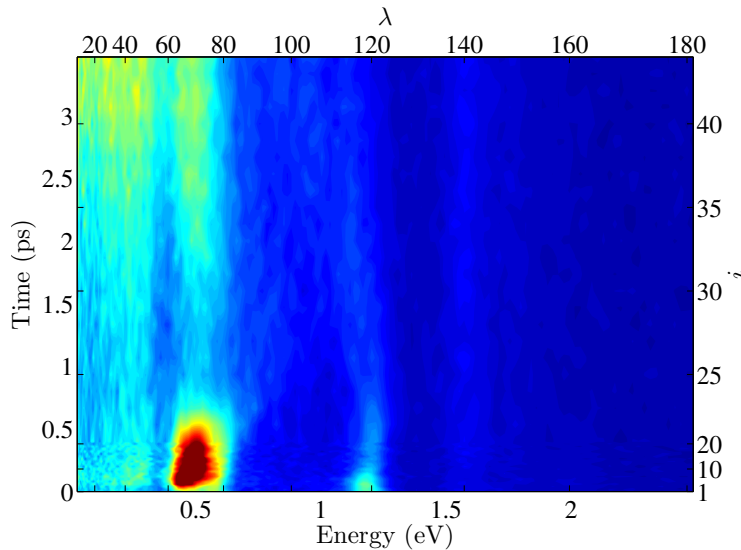
Figure 12: Photoelectron spectra ( I = 44 mixtures).
