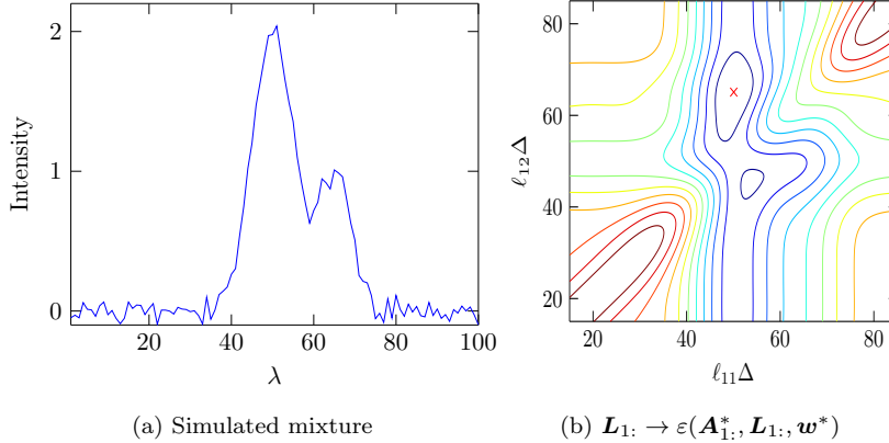
Figure 2: (a) A noisy mixture of two Gaussian sources ( I = 1, J = 2 ) with a_{11}^* = 6.0, a_{12}^* = 2.7, \ell_{11}^* \Delta = 50, \ell_{12}^* \Delta = 65, w_1^* = 5, w_2^* = 4, N = 100 . (b) The criterion \mathbf{L}_1: \rightarrow \varepsilon(\mathbf{A}_1^*, \mathbf{L}_1, \mathbf{w}^*) admits local minimizers and flat surfaces. The red \times indicates the global minimizer.
