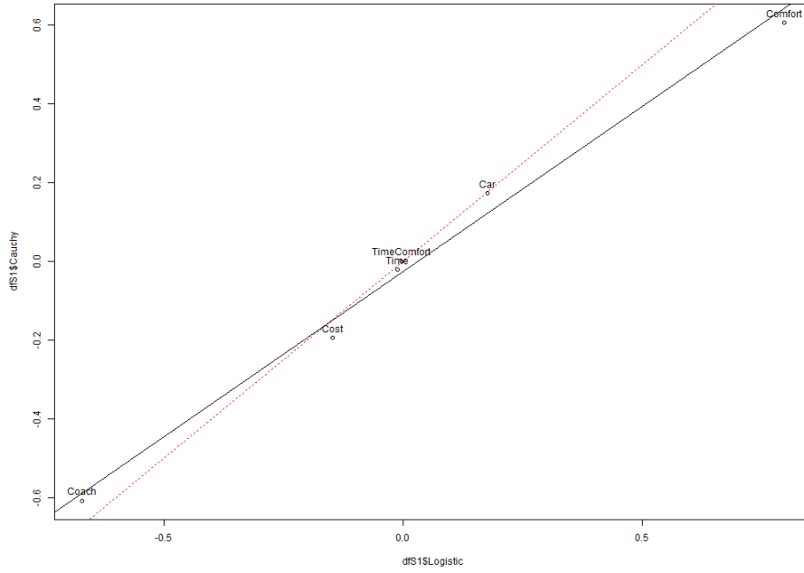
Figure 8: Coefficients Comparison - S1 - Cauchy : Logistic
