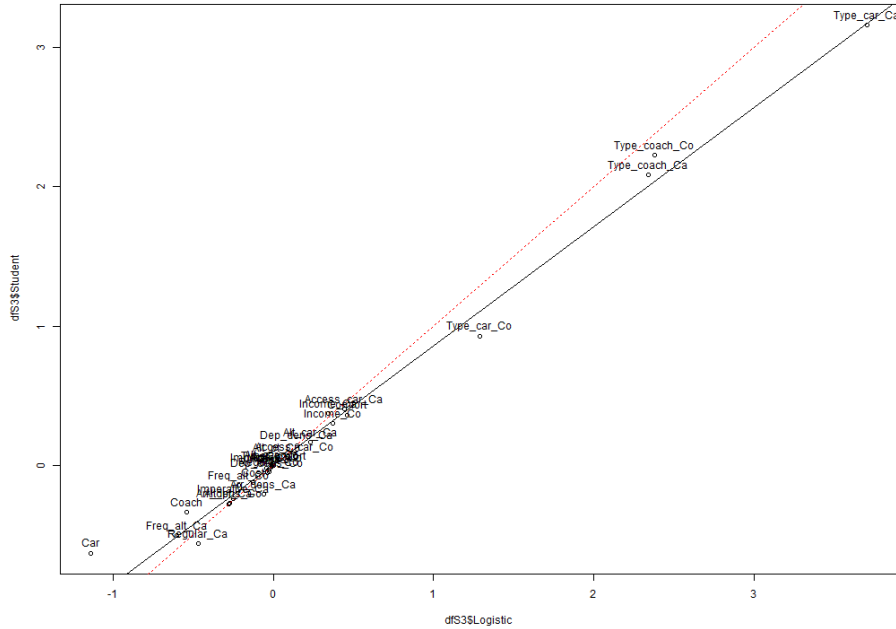
Figure 22: Coefficients Comparison - S3 - Student : Logistic
