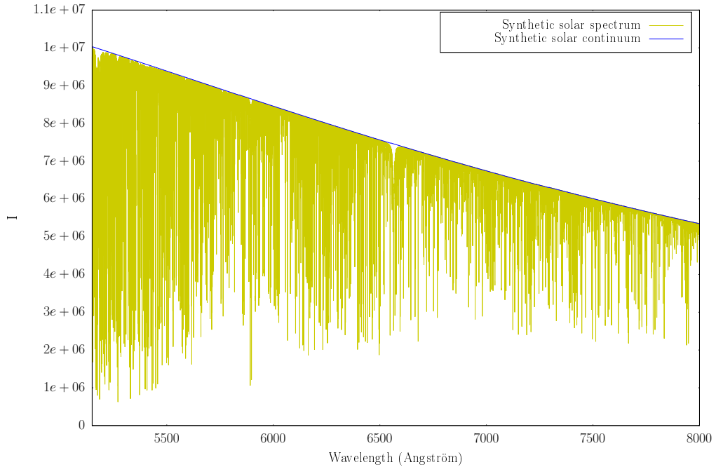
Fig. 1. Synthetic spectrum and continuum for the Sun ( T_{\text{eff}} = 5775K and \log g = 4.440 )
