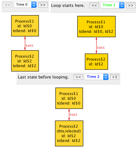
Figure 3: Example trace in the Electrum visualizer.
