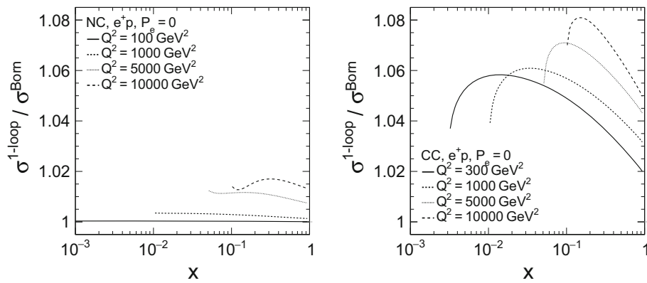
Fig. 1 Size of the purely weak one-loop corrections for the e^+ p unpolarised inclusive NC DIS (left) and CC DIS (right) cross sections at selected values of Q^2 as a function of x . QED corrections due to real and virtual photons and corrections from the vacuum polarisation (the
