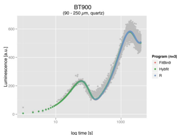
Figure 5: LM-OSL fitting using a 3-component function for the quartz sample BT900 on a log scale. The sum curves show that all programs produce similar fits and therefore the three curves are indistinguishable.
