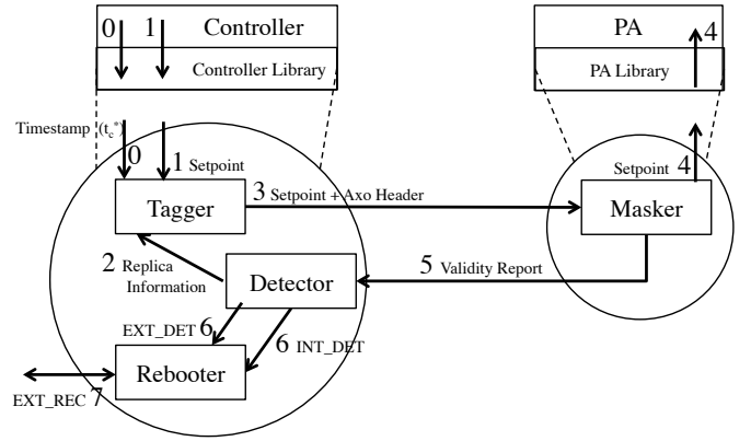
Fig. 1. Axo Architecture
