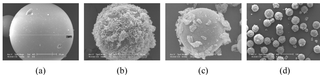
Figure 5. ESEM pictures of (a) uncoated glass bead \times 1600 , (b) glass bead coated by supercritical fluids process \times 1600 , (c) physical mixture \times 5194 , (d) general view of coated glass beads \times 200 .
