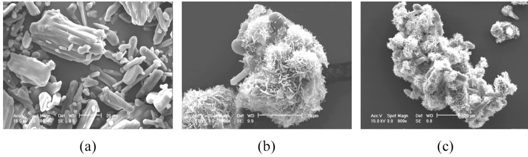
Figure 8. ESEM analysis of the (a) uncoated AC \times 800 and (b) coated AC \times 1600 , (c) \times 1900 .
