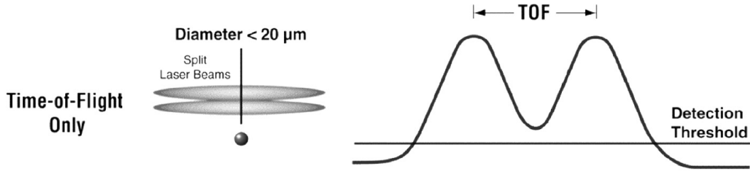
Figure 2. Time of flight detected by Aerosizer ® (TSI, USA).
