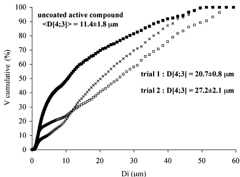
Figure 7. Cumulative volume size distribution of both uncoated and coated AC compounds vs. mean EAD.
