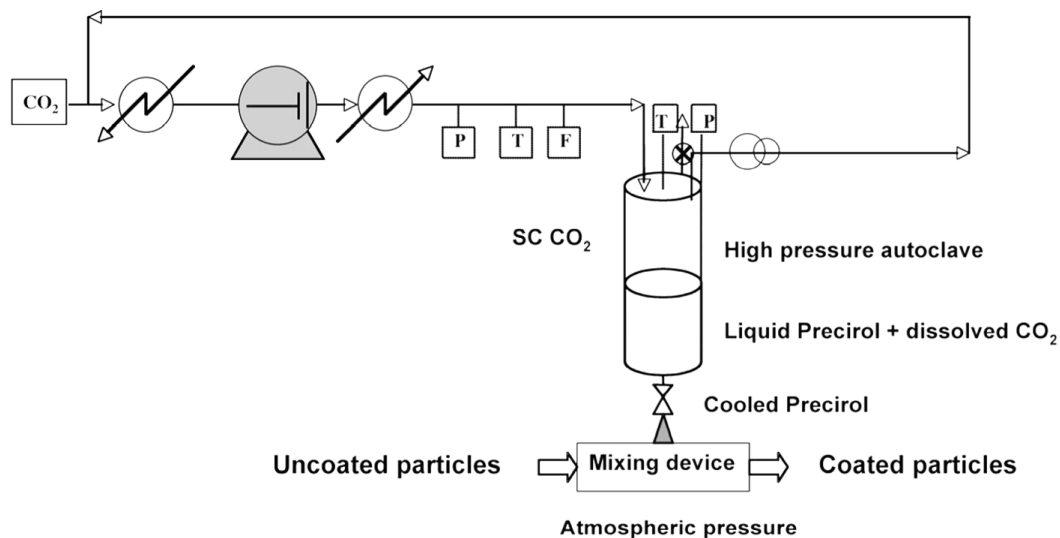
Figure 1. Experimental setup of the supercritical fluid coating process.
