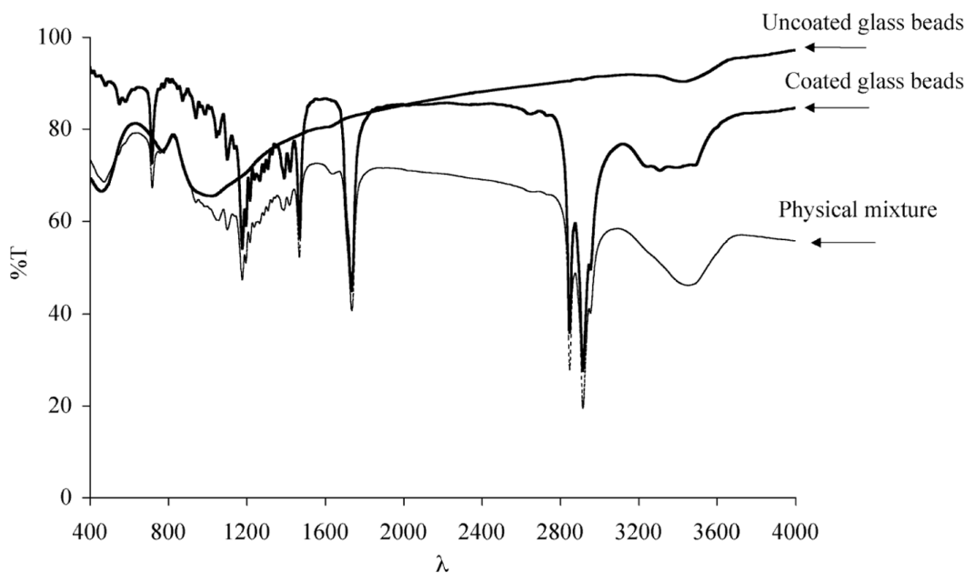
Figure 6. FT-IR spectra of the physical mixture and the coated particles.
