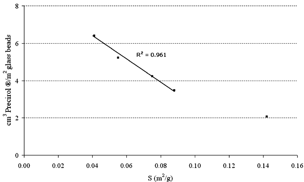
Figure 4. Volume of Precirol ® deposited onto the particles vs. specific surface area of the coated particles.
