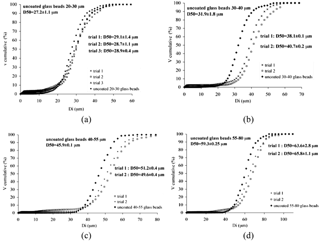
Figure 3. Cumulative percent volume versus mean diameter of the coated particles of the sieved cut glass beads by a supercritical process (a) 20–30 \mu\text{m} ; (b) 30–40 \mu\text{m} ; (c) 40–55 \mu\text{m} ; (d) 55–80 \mu\text{m} .
