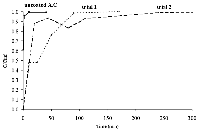
Figure 9. Test release of both coated and uncoated AC into distilled water.
