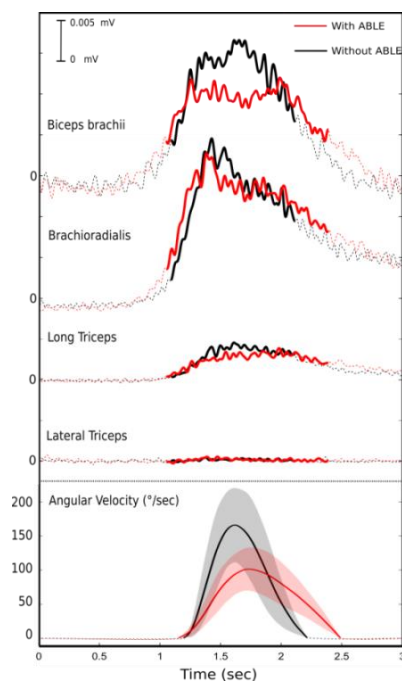
Figure 1: Smoothed-rectified EMGs of biceps brachii, brachioradialis, long and lateral heads of triceps brachii, and corresponding angular velocity ( \pm SD) during an elbow flexion with/without exoskeleton.
