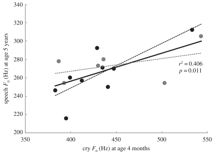
Figure 1. Relationships between the mean F_0 of babies' cries around 4 months of age and the mean F_0 of their speech around the age of five years. Boys ( n = 9 ) are represented as black dots and girls ( n = 6 ) as grey dots. Dotted lines represent trendlines for each sex. Statistics are reported for the pooled-sex trendline (solid black).
