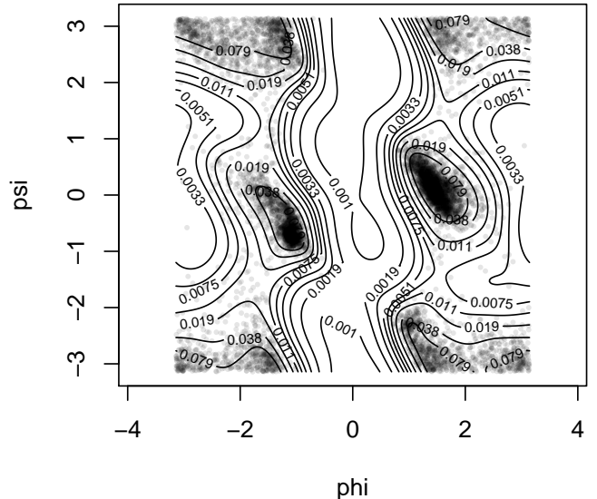
Figure 4: Each point represents two dihedral angles for a Glycine amino acid. These angles are used to describe the global three dimensional shape of a protein. They live on the bitorus. The level sets are those of the empirical Christoffel functions evaluated on the sphere in \mathbb{R}^4 . The degree is 4.
