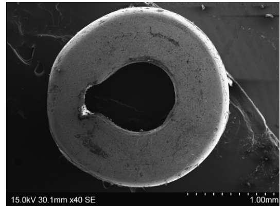
Fig. 9. SEM image of the microbead from El Chorro de Maíta. Note the faint traces of the seam to the left of the image (photograph by Marcos Martínón-Torres and Roberto Valcárcel Rojas).
