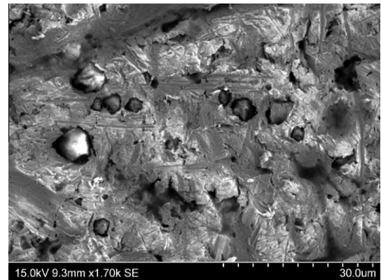
Fig. 10. SEM detail of the surface of the microbead from El Chorro de Maíta, showing abundant quartz inclusions (photograph by Marcos Martínón-Torres and Roberto Valcárcel Rojas).
