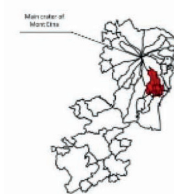
Fig. 1. Spatiotemporal cluster identified by Kulldorff's spatial scan statistics in the Mount Etna region.
