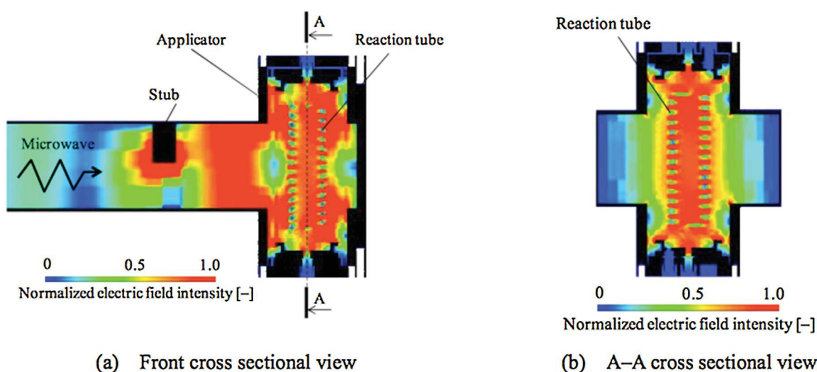
Fig. 5. Simulation of the electric field intensity in the waveguide [45].
