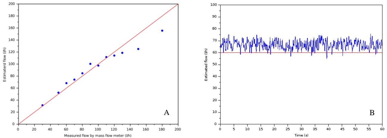
Figure 2. Methane flow estimation (blue) and reference (red) at the laboratory: (A), Mean flow estimation for several leakage rates; (B), Instantaneous flow estimation for one leakage rate.
