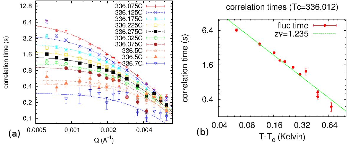
FIG. 5. (a) Fluctuation times \tau(q, T) for various temperatures and the lorentzian fits. (b) Temperature variations of \tau_0(T) . An estimate of the exponent yielded z\nu = 1.235(70)
