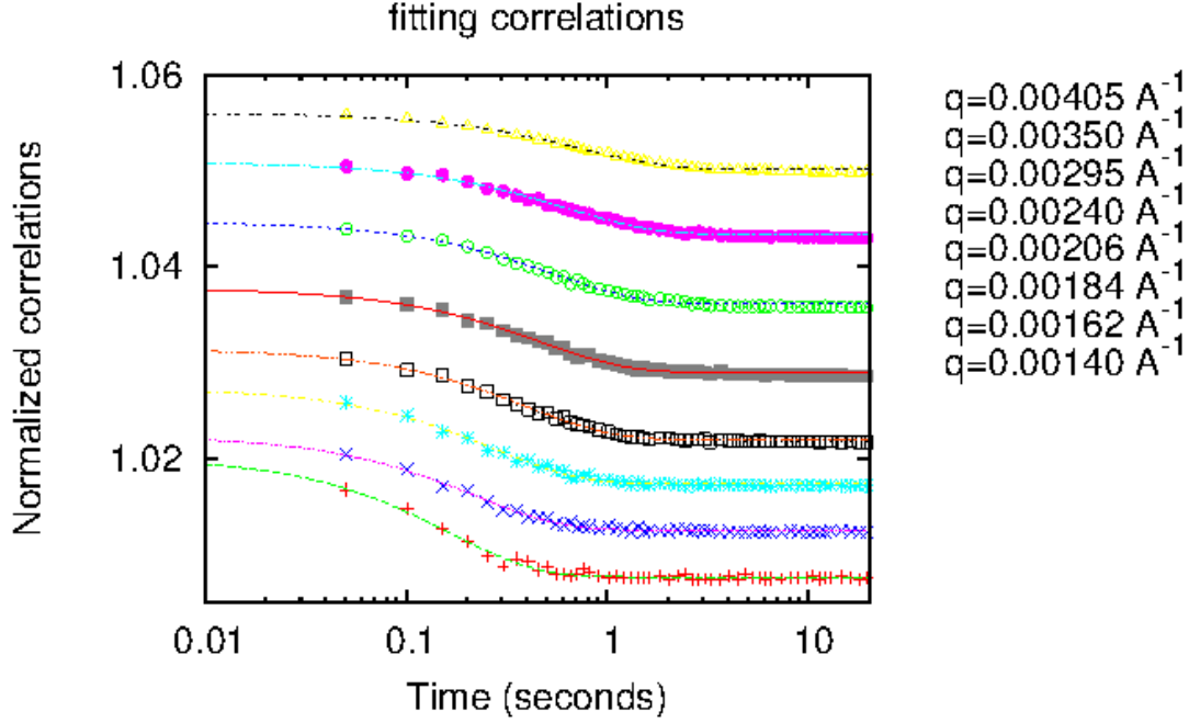
FIG. 4. Time correlations obtained for various q vectors at T=T_c+0.113\text{K} . Curves are shifted vertically for sake of visibility. Symbols correspond to values of the g_2(q, t) function and solid lines to a least-square fits with Eq. 3
