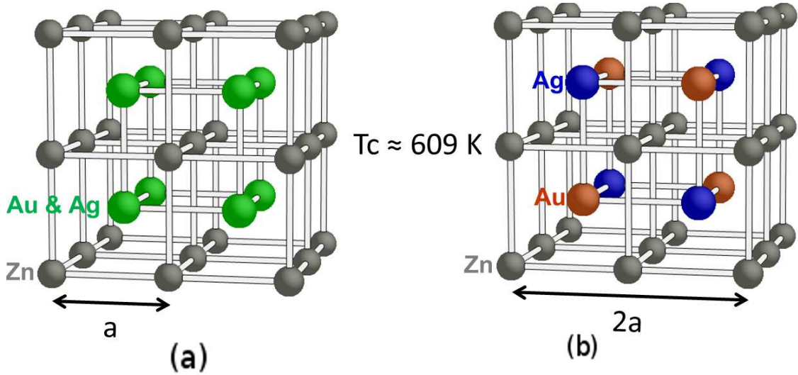
FIG. 1. (a) B2 and (b) L2_1 ordered structures of the \text{AuAgZn}_2 alloy near T = 609 \text{ K} . The lattice parameter a of the B2 phase is close to 3.17 \text{ \AA} at 603 \text{ K} .
