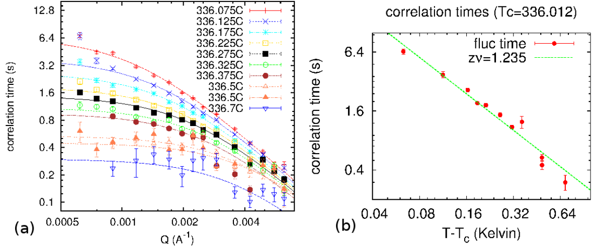
FIG. 5. (a) Fluctuation times \tau(q, T) for various temperatures and the lorentzian fits. (b) Temperature variations of \tau_0(T) . An estimate of the exponent yielded z\nu = 1.235(70)
