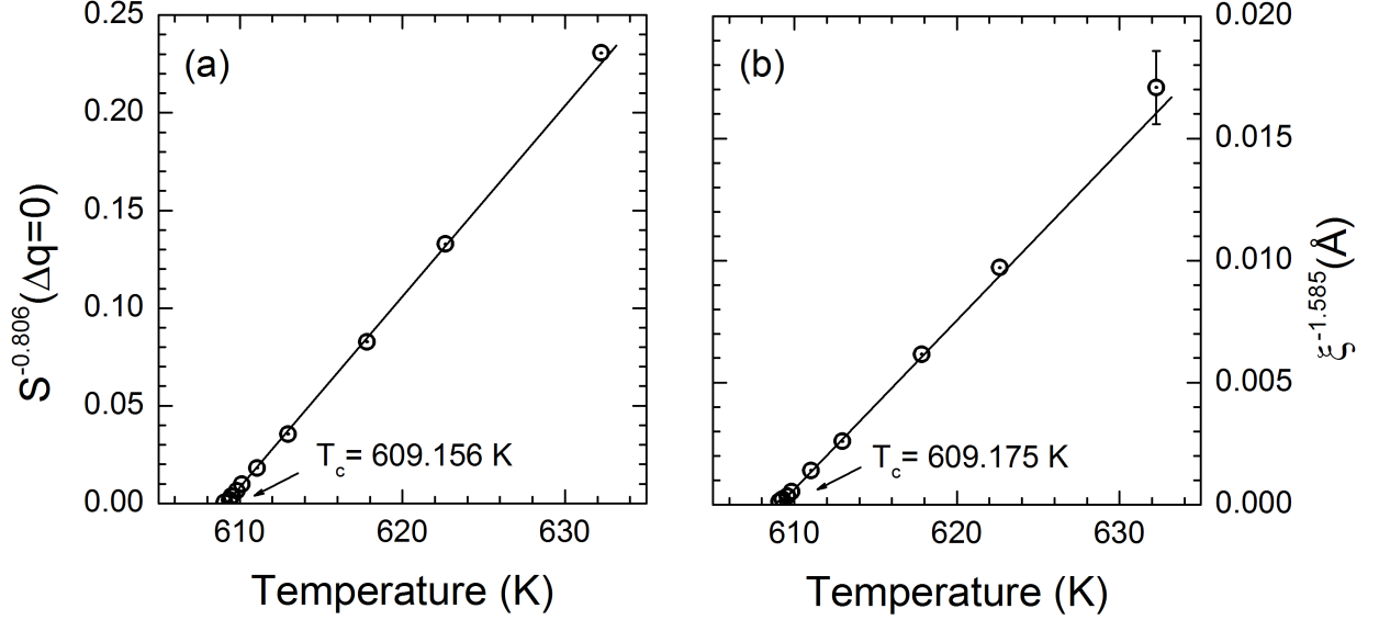
FIG. 3. Determination of the critical temperature by fitting intensity profiles to Eq. 2. (a) from the variation of S^{-1/\gamma}(q=0) with \gamma=1.241 . (b) from the variation of \xi^{-1/\nu} with \nu=0.63 .
