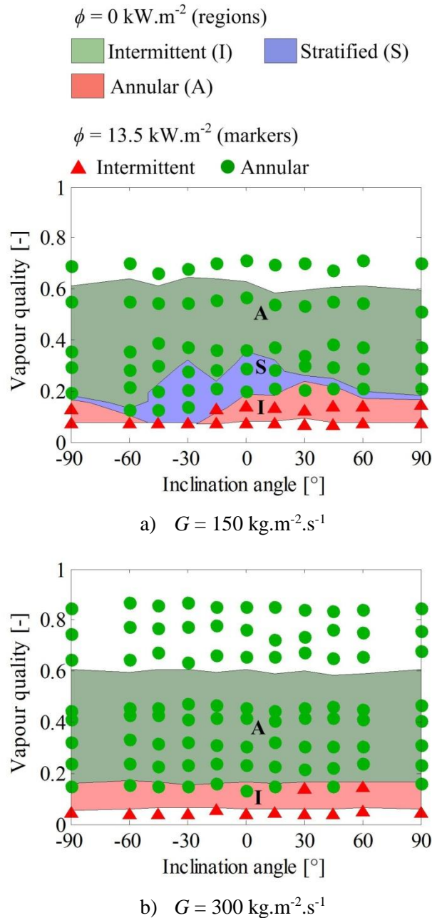
Figure 8: Variations of the flow patterns with \phi = 13,5 \text{ kW.m}^{-2} compared to the adiabatic conditions
