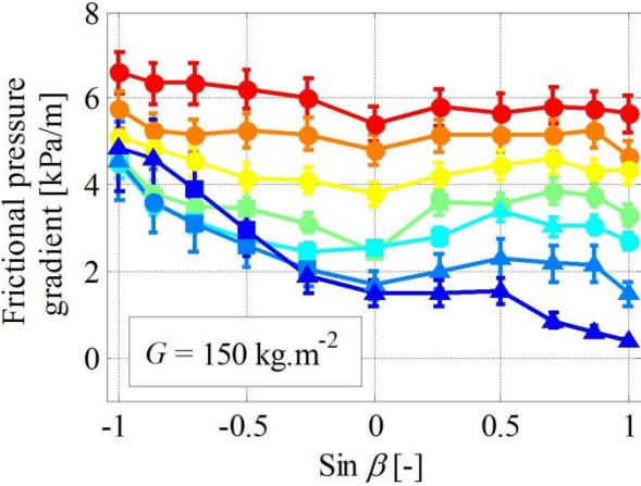
b) Frictional pressure gradient
