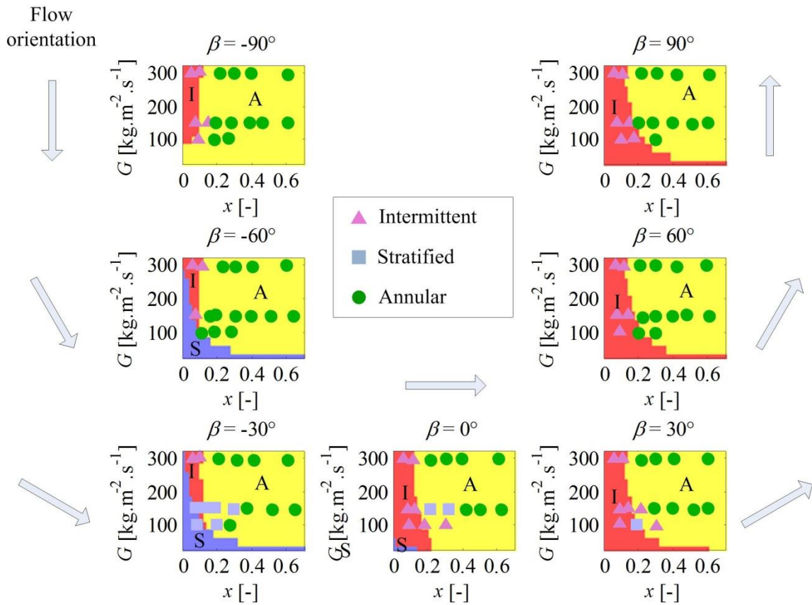
Figure 5: Comparison of experimental flow patterns with Barnea [4] flow pattern maps
