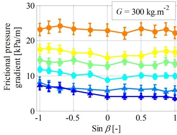
d) Frictional pressure gradient
