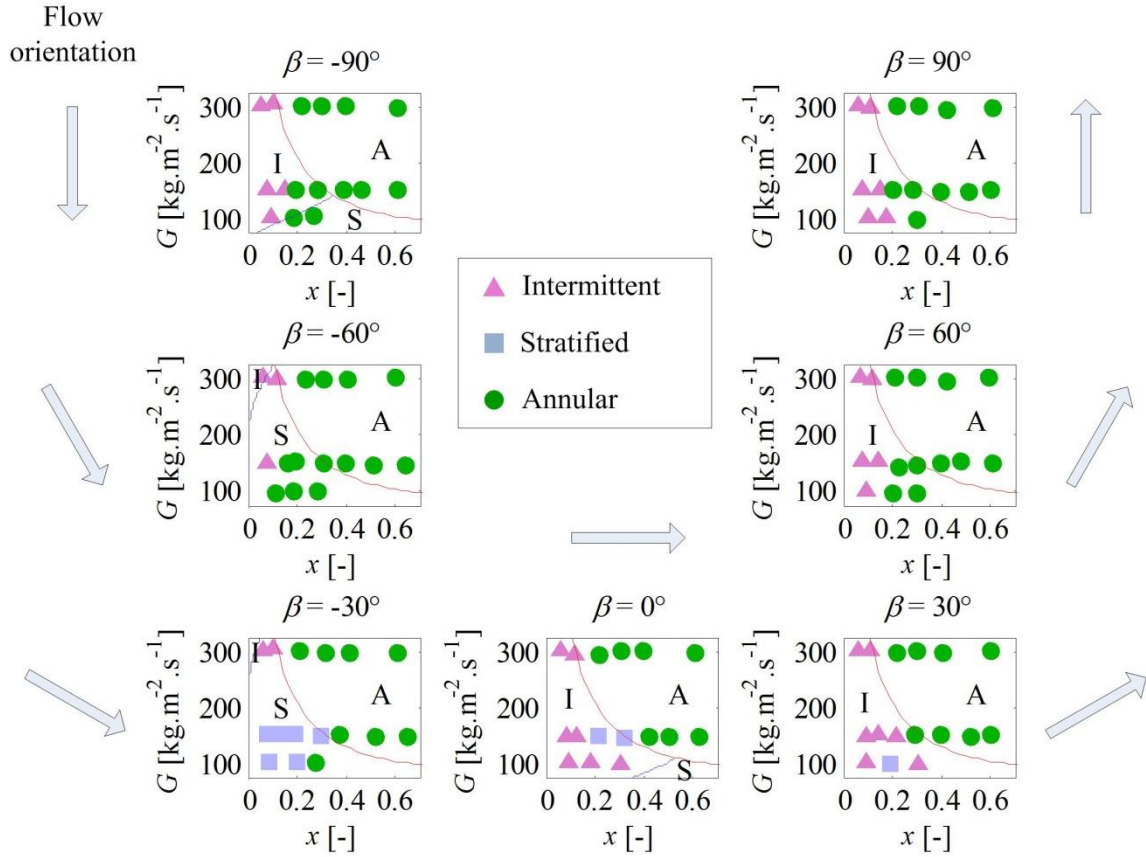
Figure 6: Comparison of experimental flow patterns with Crawford et al. [5,6] flow pattern maps
