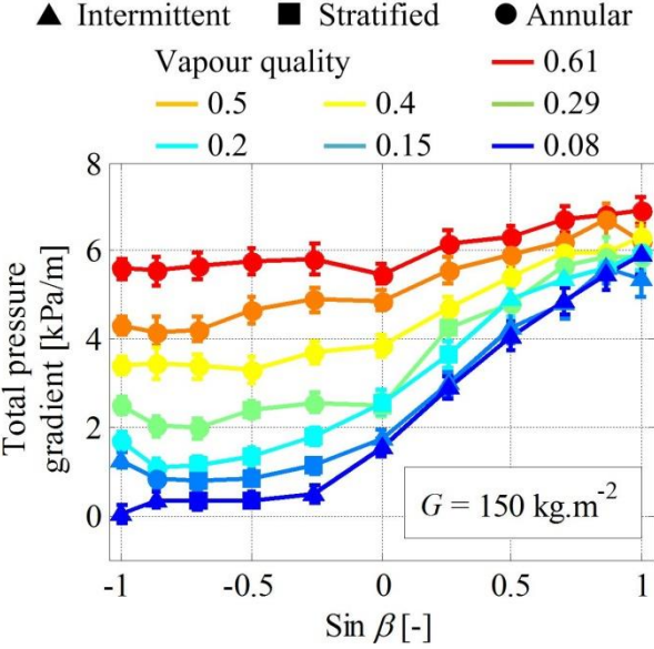
a) Total pressure gradient
