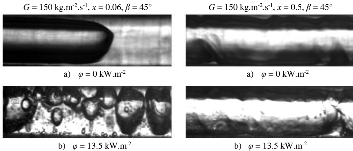
Figure 7: Example of the heat flux effect on the flow pattern ; representative frames of the flow without heat flux (a) and with a heat flux of 13,5 kW.m -2 (b)
