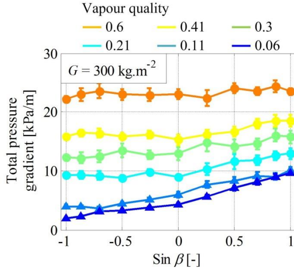
c) Total pressure gradient
