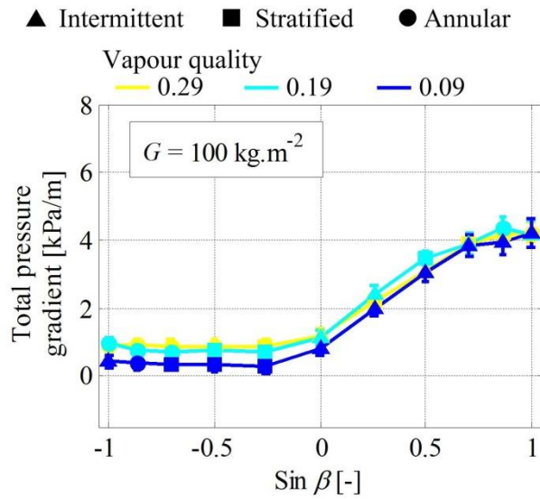
a) Total pressure gradient
