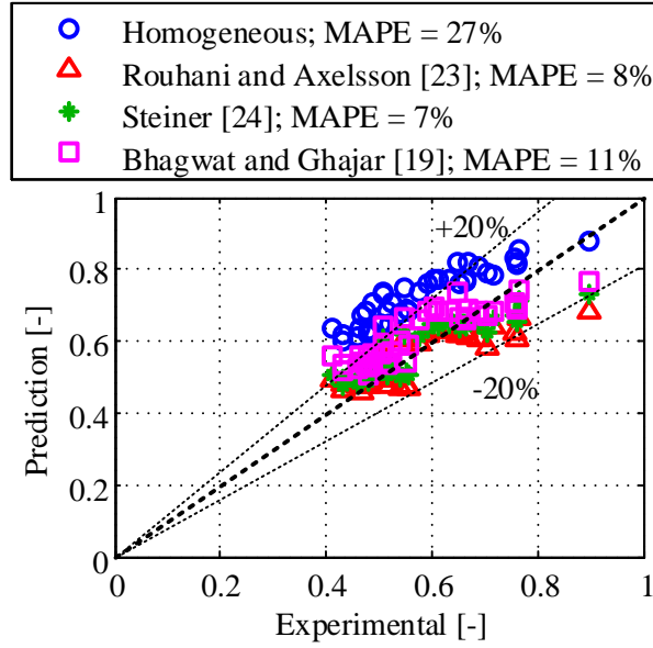
Figure 10: Statistical analysis of the void fraction models
