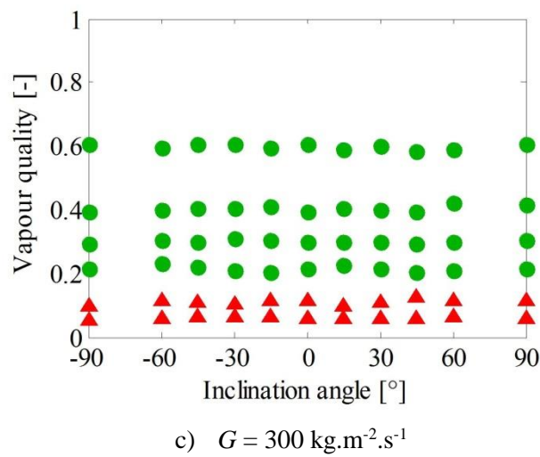
Figure 4: Variations of the flow patterns with the vapour quality and the inclination angle with G = 100 \text{ kg.m}^{-2}.\text{s}^{-1} (a), G = 150 \text{ kg.m}^{-2}.\text{s}^{-1} and G = 300 \text{ kg.m}^{-2}.\text{s}^{-1} (c) ( \varphi = 0 \text{ kW.m}^{-2} )
