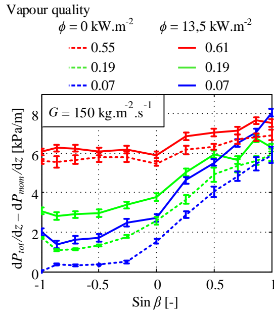
Figure 15: Comparison of the pressure gradient variations with the inclination angle with an imposed heat flux of 13.5 \text{ kW}\cdot\text{m}^{-2} (filled lines) and without heat flux (dot lines)
