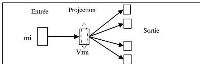
FIGURE 2 : Architecture Skip-Gram
