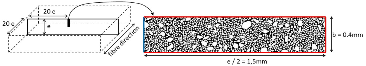
Figure 5. Mechanical and hydric boundary conditions.
