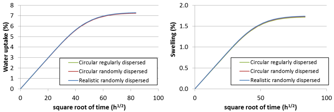
Figure 6. Water uptake and thickness swelling of the 3 FEM models.
