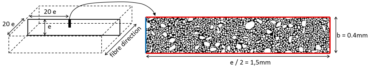
Figure 5. Mechanical and hydic boundary conditions.
