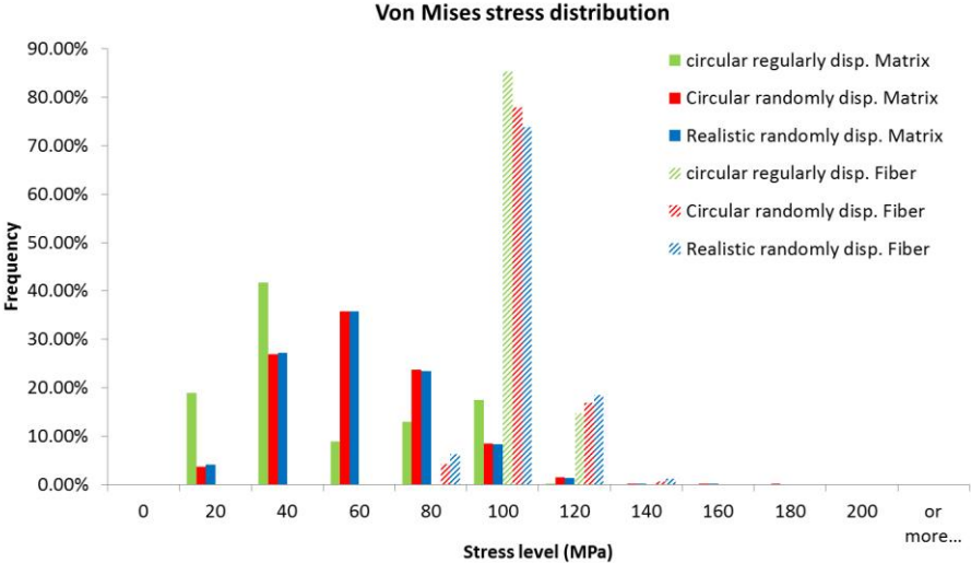
Figure 8. Stress distribution in matrix and fibers at saturation (7000h) of 3 flax/polyester composites FEM.
