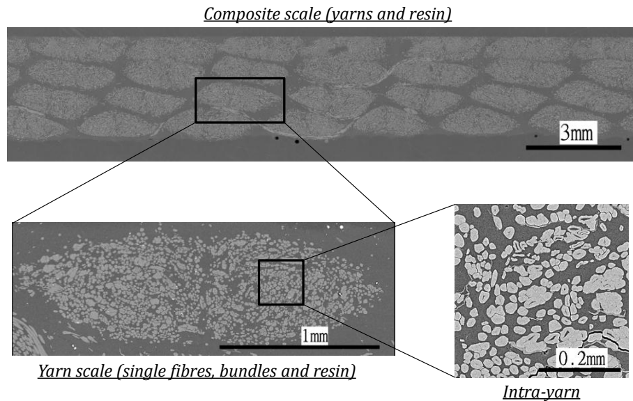
Figure 1 - Multiscale microstructure of the unidirectional flax fiber reinforced polyester
