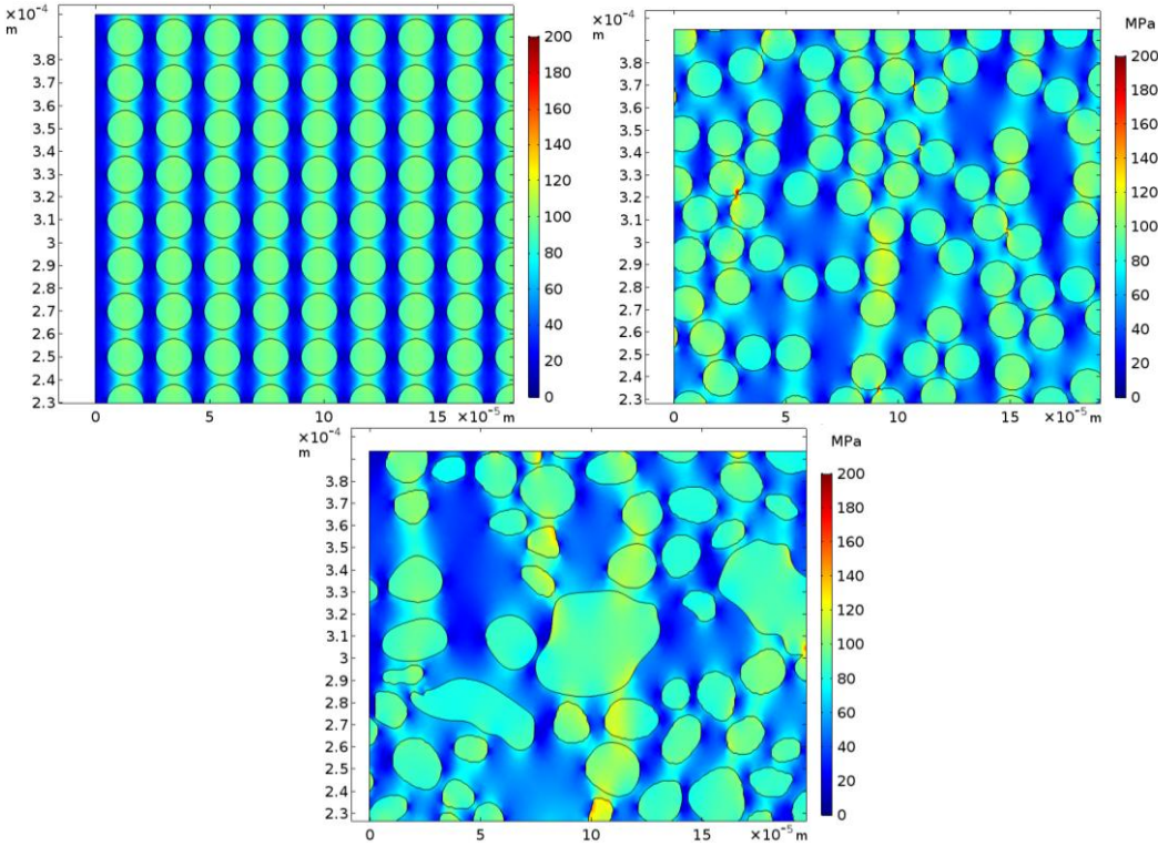
Figure 7. Stress distribution in MPa at saturation (7000h) of 3 flax/polyester composites FEM.
