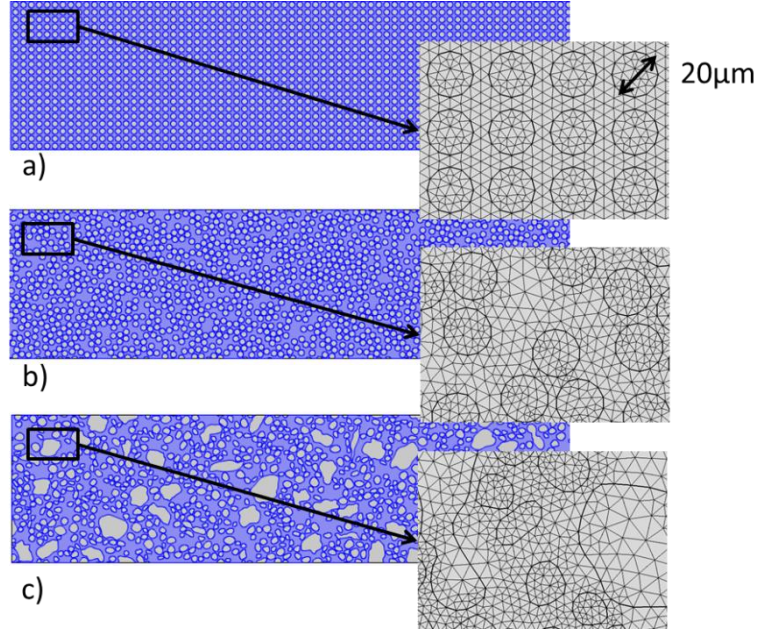
Figure 4. Examples of generated microstructures ( V_f=46-47\% ) – a) Regularly dispersed circular fibers – b) Randomly dispersed circular fibers – c) Randomly dispersed statistically representative fibers.
