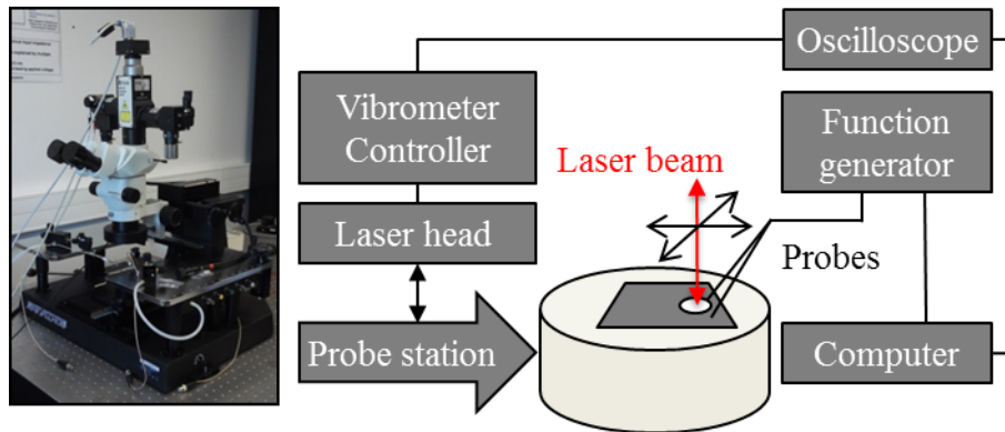
Figure 3 Laser setup
