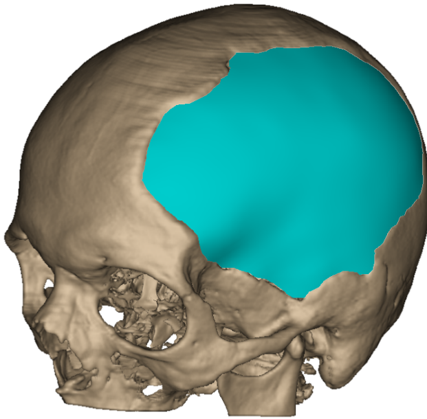
Fig. 11 Exterior implant surface after boundary fitting.
