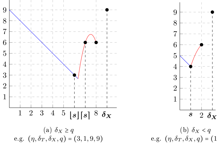
Figure 9: Examples of graph of the function f when \max\left(\frac{\delta}{\eta+1}, \delta_T\right) < q \leq \delta
