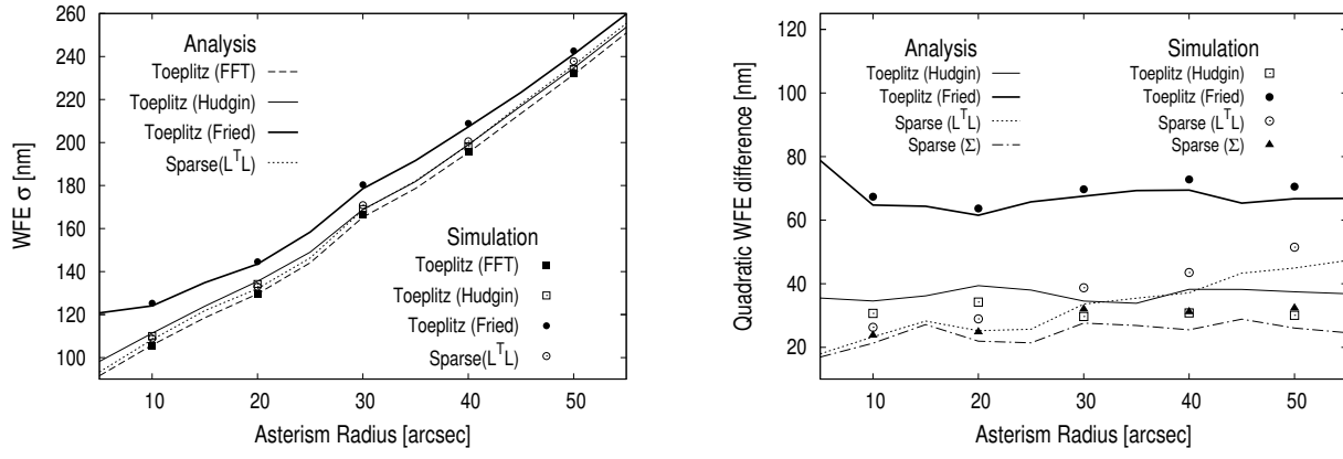
Fig. 9. Left: WFE with different algorithm as function of asterism of guide stars. The lines shows the analytical results and the points shows the results from numerical simulation. Right: Quadratic WFE difference from the WFE of the Toeplitz method with the FFT gradient model. The symbols are the same as those in the left panel, except for the dot-dashed line and triangles showing the result with the sparse method with non-approximated real regularization term.
