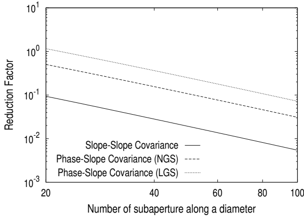
Fig. 8. Reduction factor of the number of operations required for \Sigma_{ss}\zeta (solid line) and \Sigma_{\phi s}\zeta (the dashed line for NGSs case and the dotted line for LGSs case) as function of the number of subapertures across telescope diameter, assuming N_{gs} = 6 , N_{layer} = 9 and n' = 1.2n ( h_{lgs} = 90 km and h_{N_{layer}} = 16 km). The coefficient for the FFT is assumed a = 5 .
