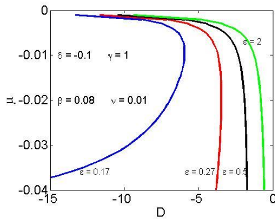
Figure 4. Resonance curves in the (D, \mu) plane found by the collective variable approach for different values of nonlinear gain \varepsilon = 0.17 (blue), \varepsilon = 0.27 (red), \varepsilon = 0.5 (black) and \varepsilon = 2 (green). Other CGLE parameters appear inside the Figure.
