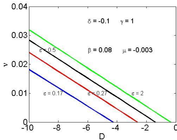
Figure 5. Resonance curves in the (D, \nu) plane found by the collective variable approach for different values of nonlinear gain \varepsilon = 0.17 (blue), \varepsilon = 0.27 (red), \varepsilon = 0.5 (black) and \varepsilon = 2 (green). Other CGLE parameters appear inside the Figure.
