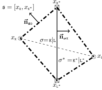
Figure 3: A diamond d = d_{\sigma, \sigma^*} with \sigma \subset \mathcal{E}_{int}
